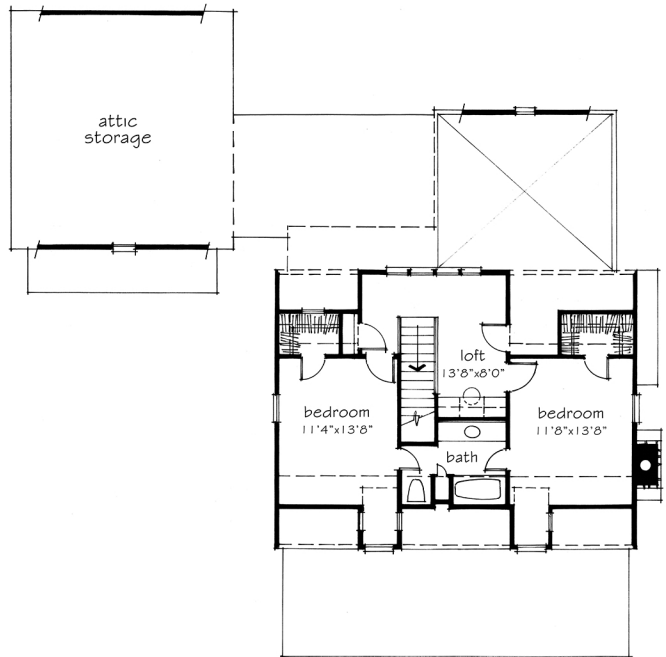
SECOND LEVEL (653 heated sq.ft.) 9' ceiling ht. Five Forks: Second Floor Plan
